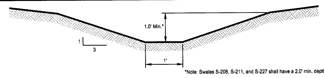
Typical Swale Cross Section
