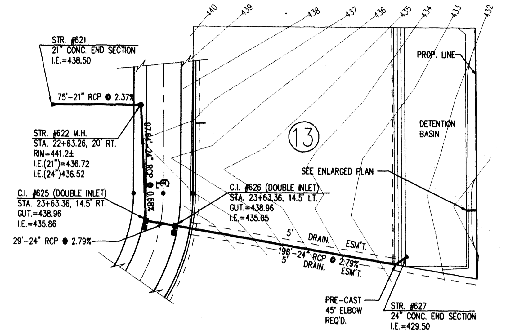
STORM "C" - PLAN VIEW SCALE: 1"=50'
