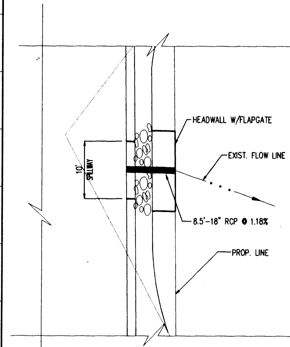
ENLARGED PLAN SCALE: 1"=10'
