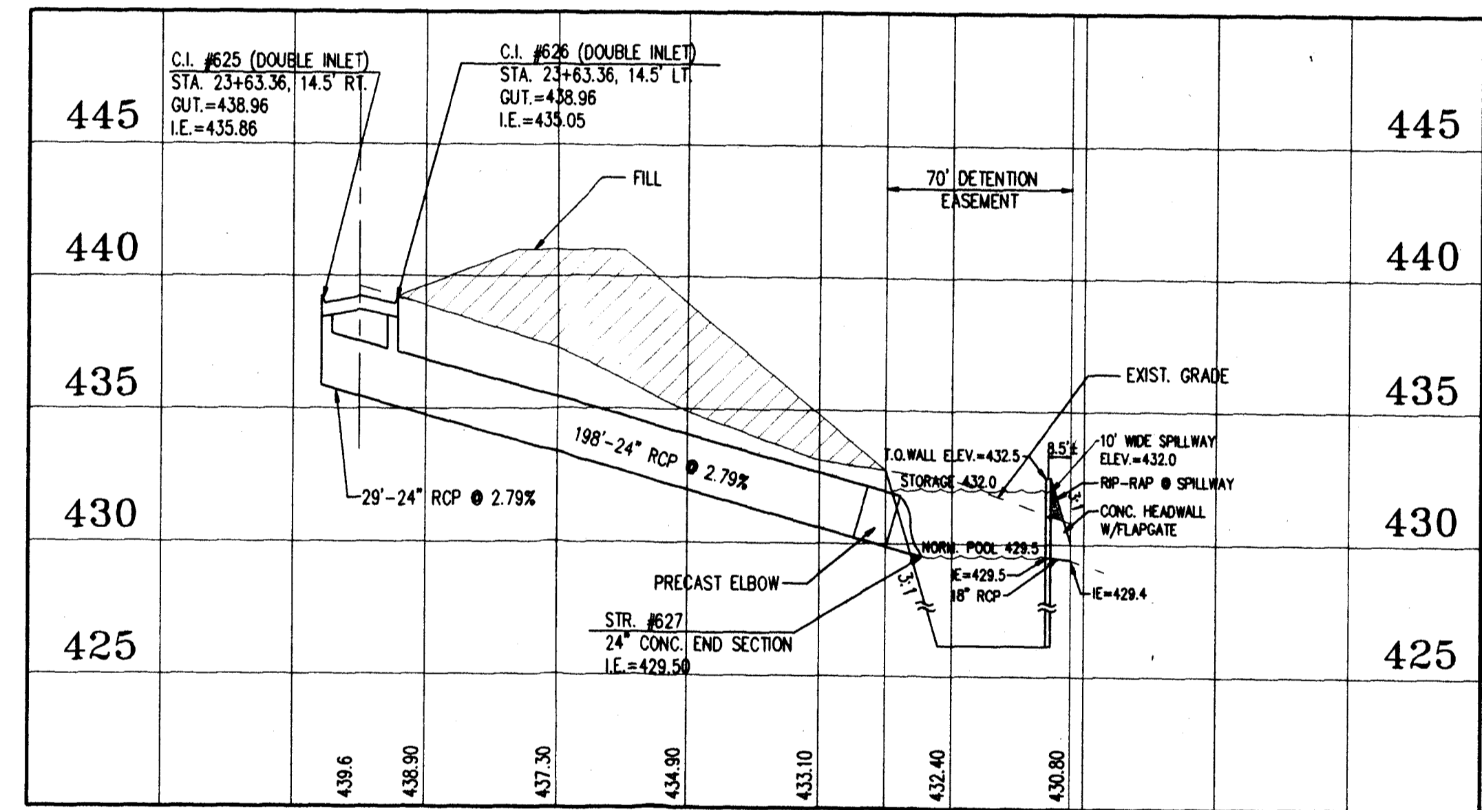
STORM PROFILE "C" SCALE: 1"=50'
