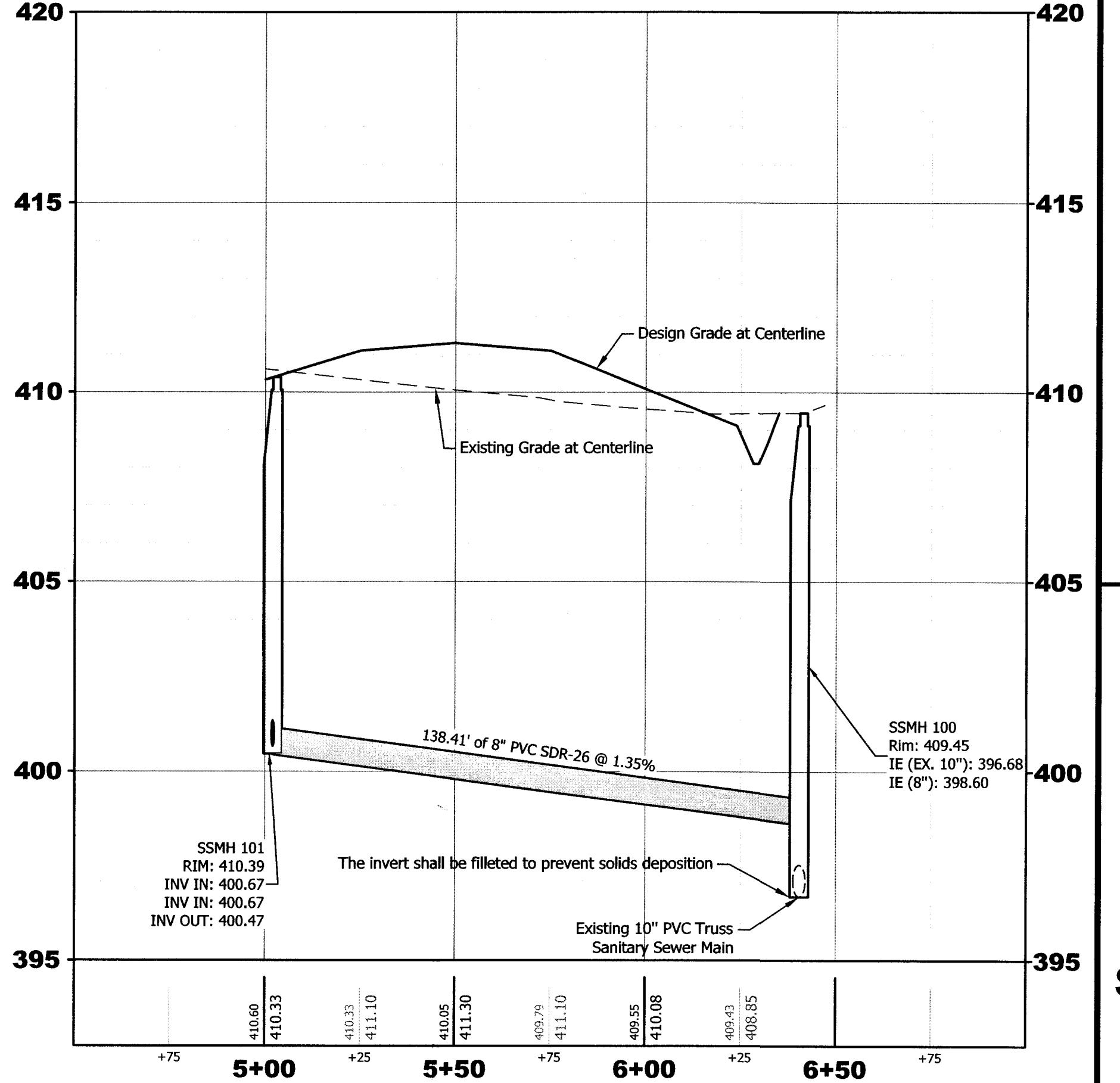
Sanitary Sewer Line A Profile
