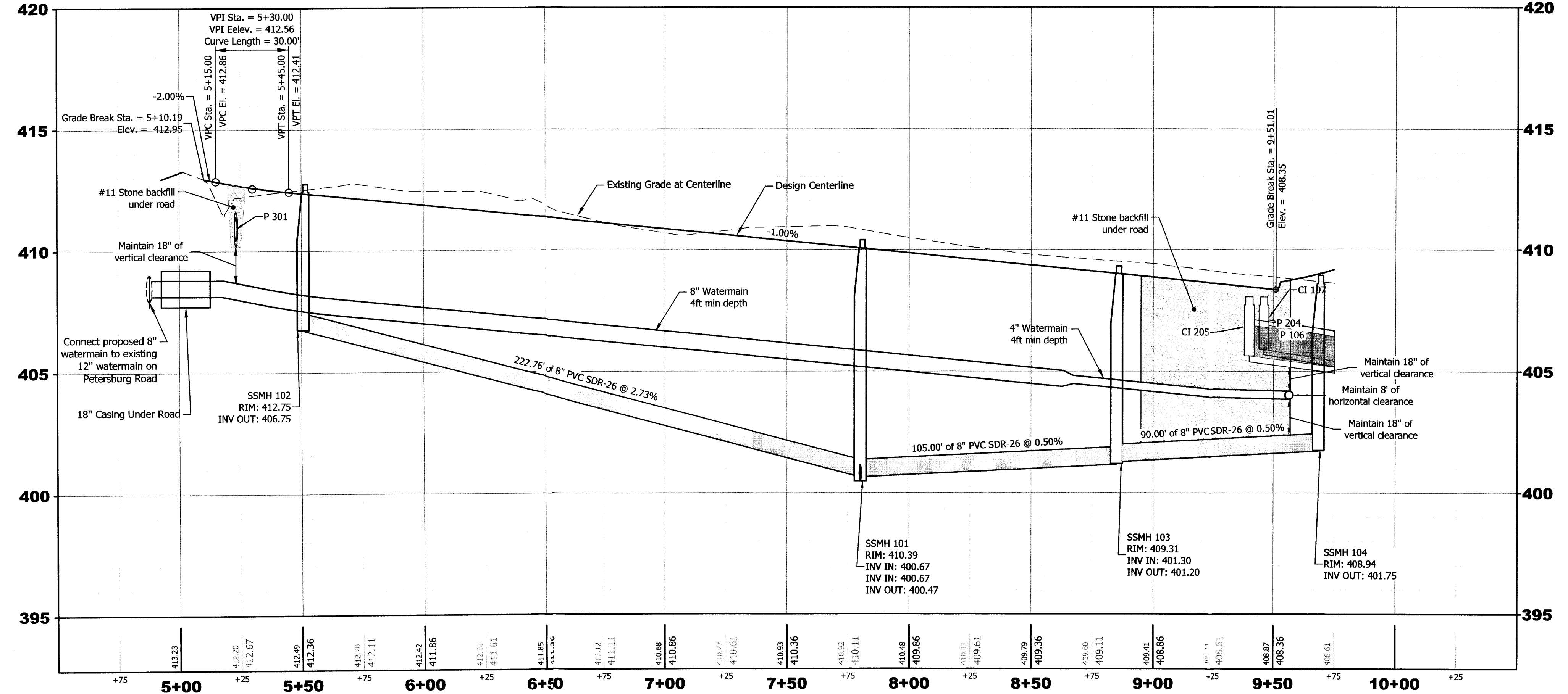
Road 1 Profile
