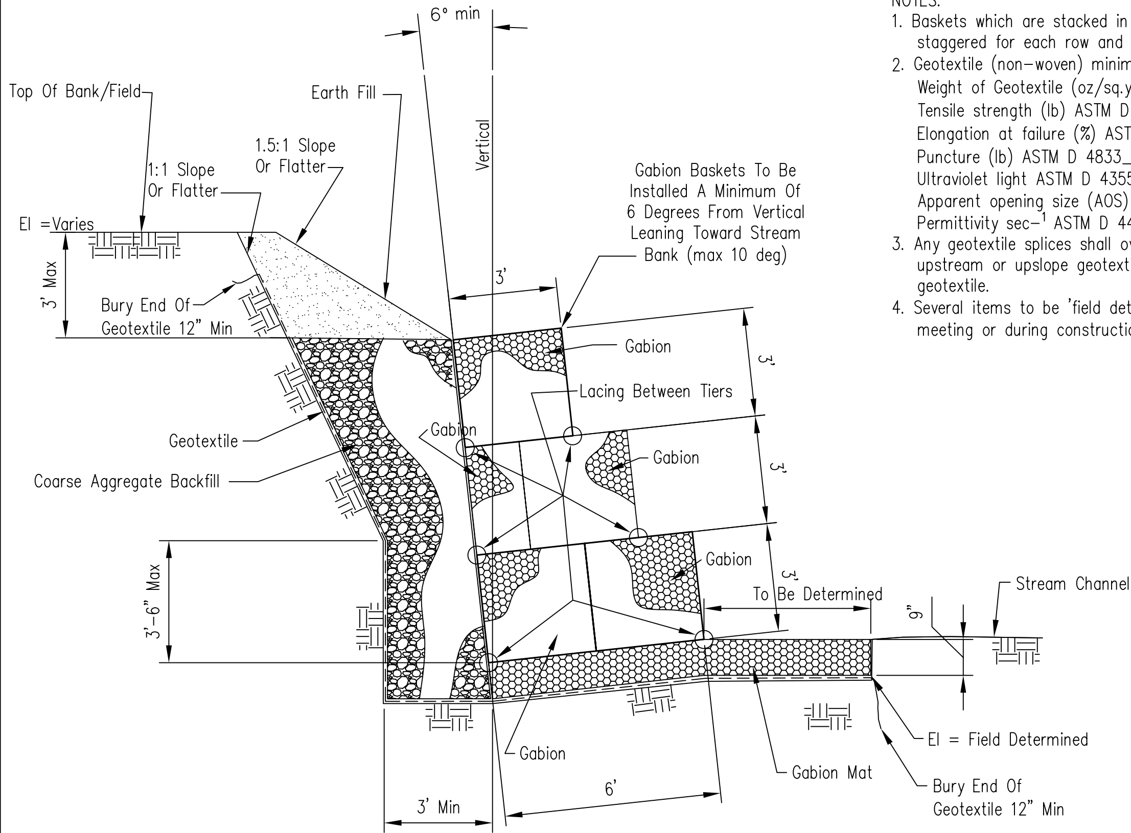
TYPICAL SECTION
